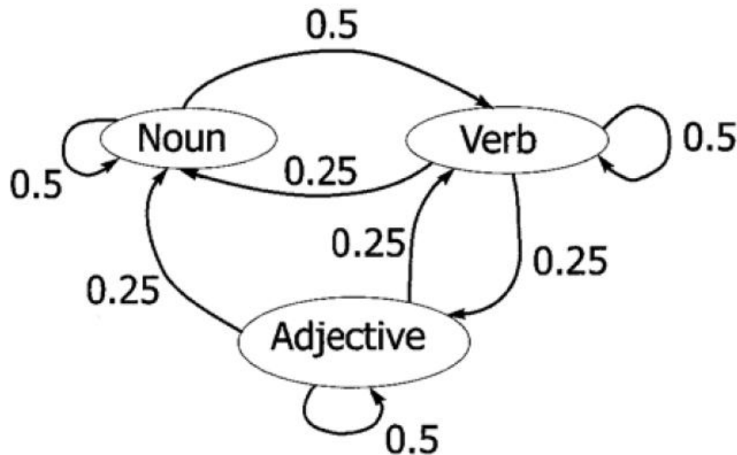
FIGURE 2.7 Transition probabilities for three parts of speech.
