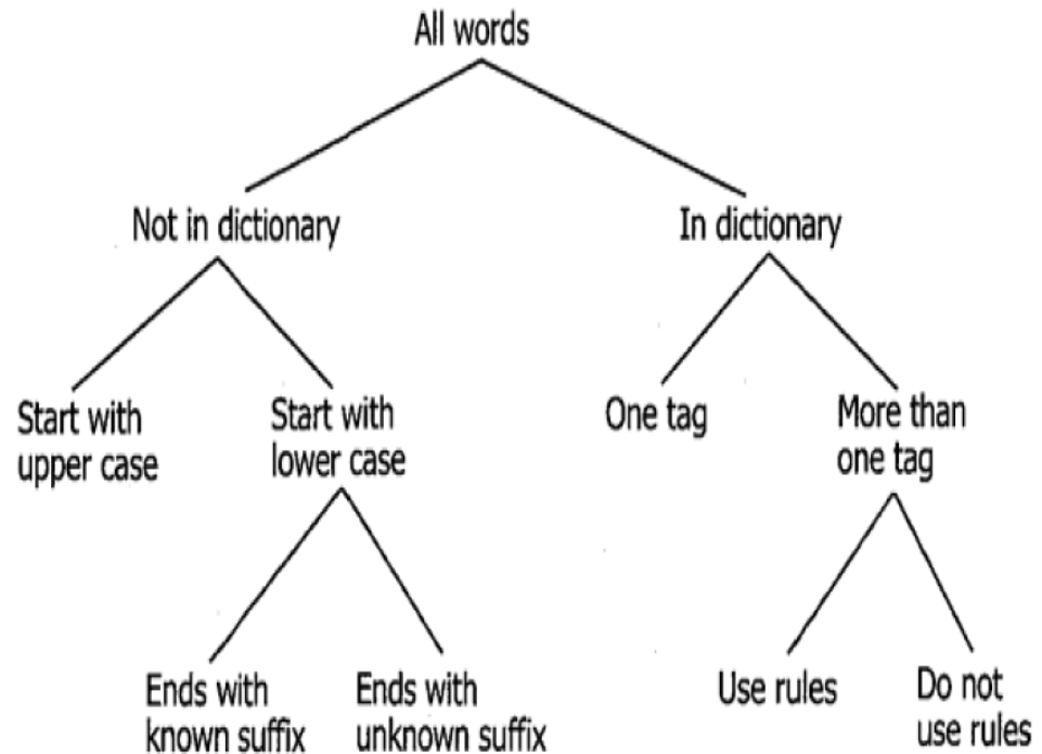
FIGURE 4.9 Decision tree to assign POS tags.
